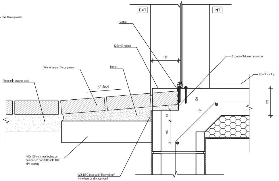
STEEL WINDOW SILL DETAIL
