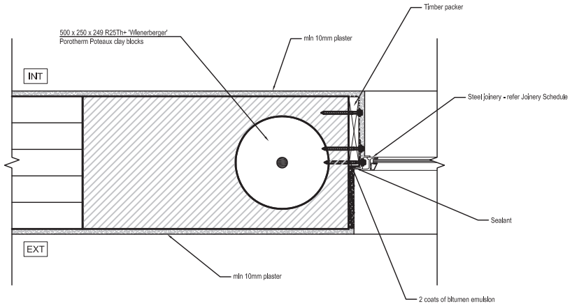
STEEL WINDOW / DOOR JAMB DETAIL
