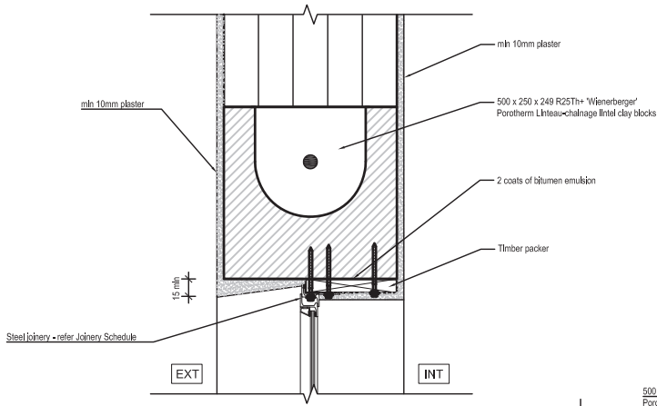
STEEL WINDOW / DOOR HEAD DETAIL
