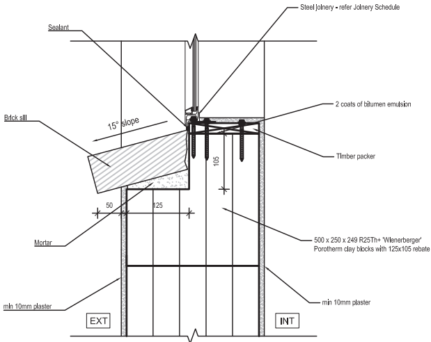
STEEL WINDOW SILL DETAIL
